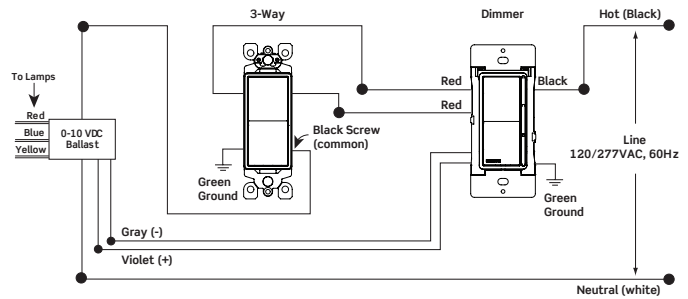
3-Way
