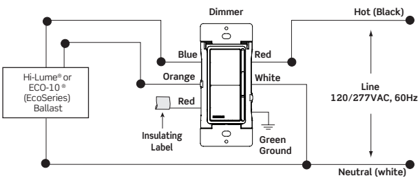
Single Pole
